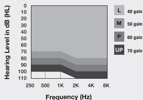
RIC with Custom Cased Receiver
